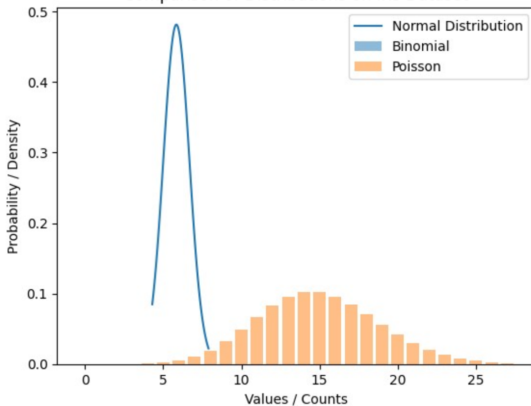
Comparison of Distributions on Iris Dataset
